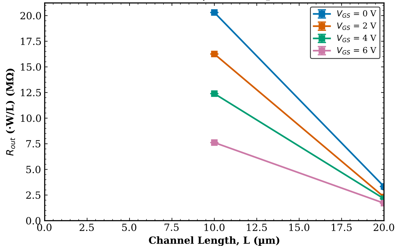
TFT3 Transistor 2 R_{out} vs L | W = 50\text{ }\mu\text{m}
